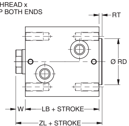
Style MR Metric Tapped Both Ends Mount with Pilot Cap
