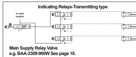
Transmitting Relay Circuit (system in mode A - working range)
