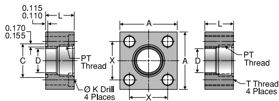
O-ring Face
