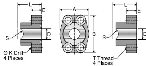
O-ring Face
